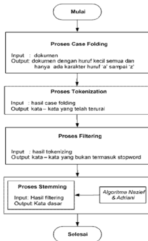
Gambar 1 Flowchart Preprocessing
