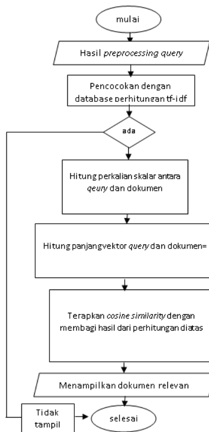
Gambar 2 Flowchart Cosine Similarity
