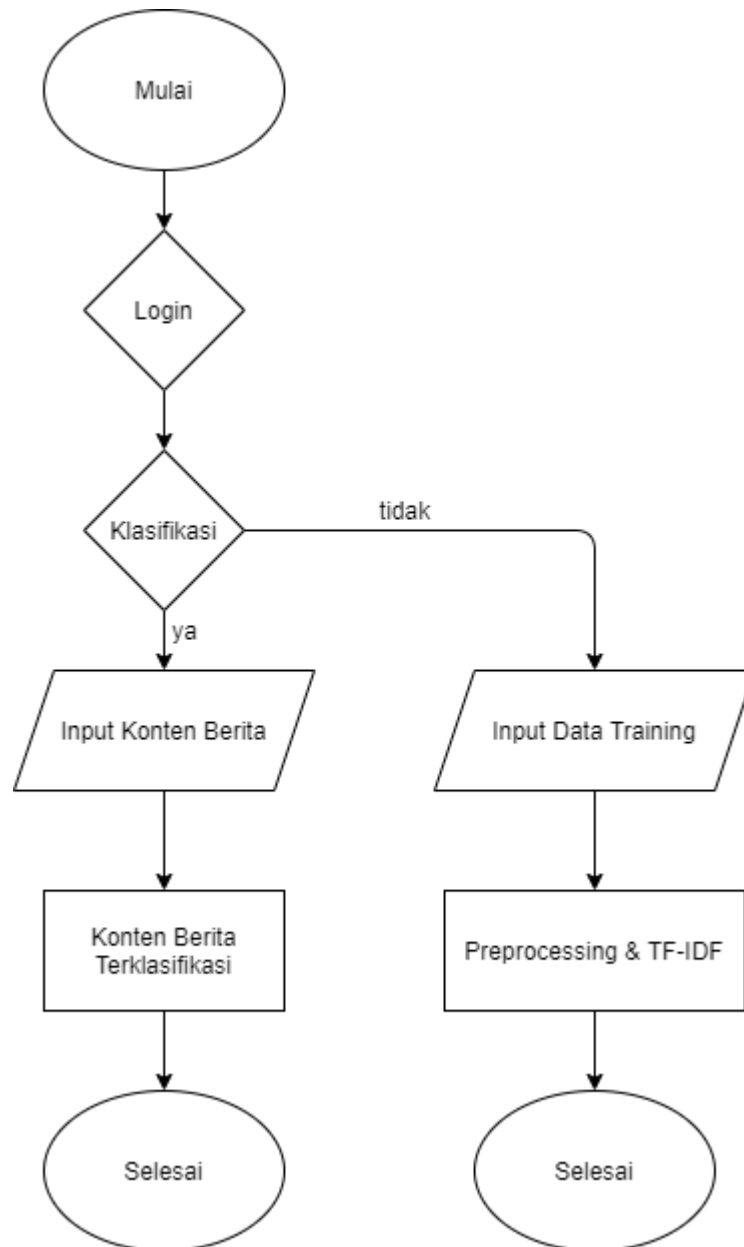
Gambar 3 Flowchart sistem
